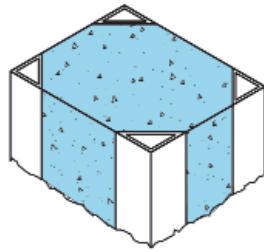
Chamfer Formers and Column Chamfer Formers
